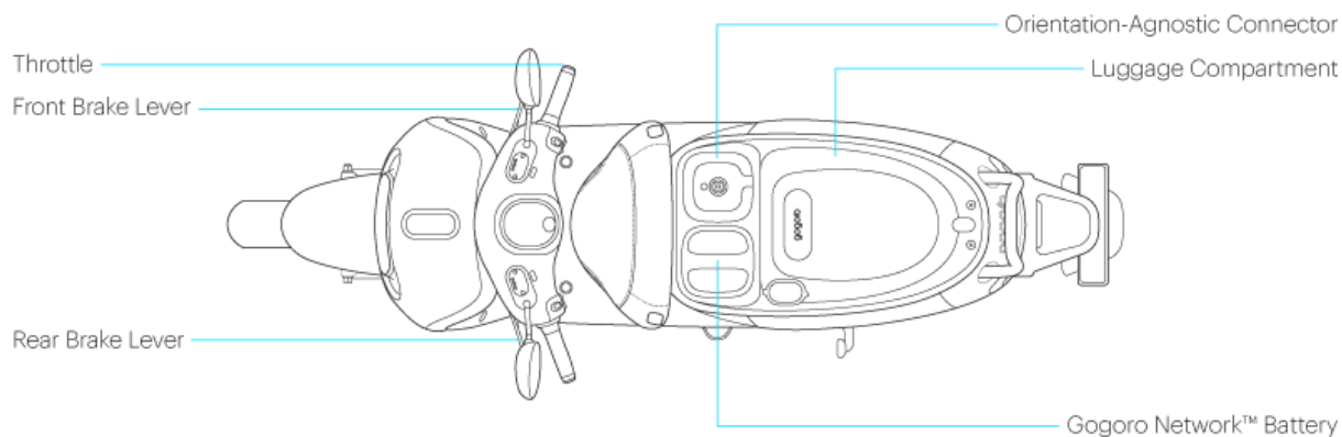
Top View
