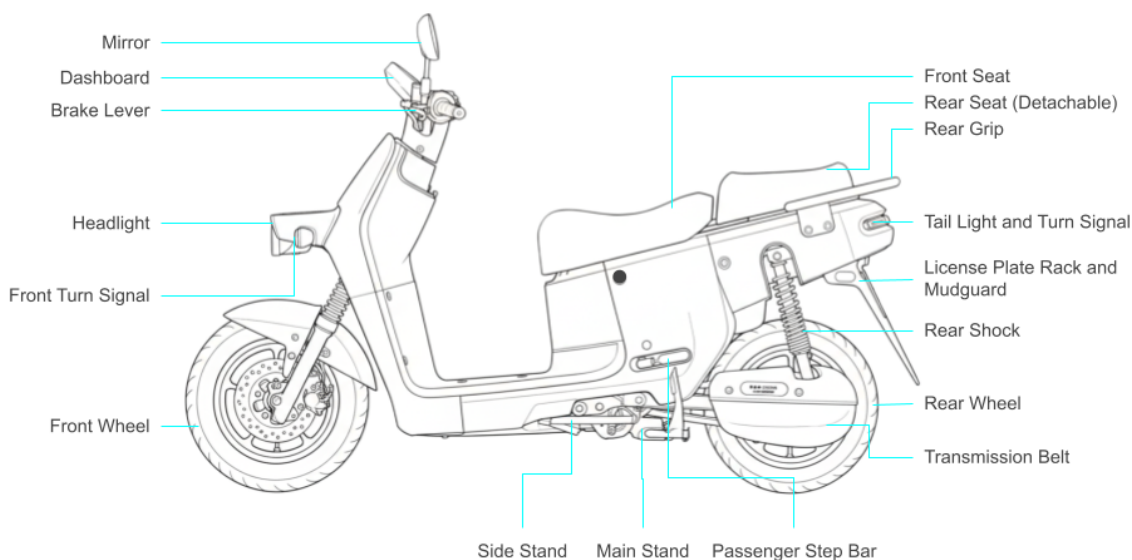
Left View
