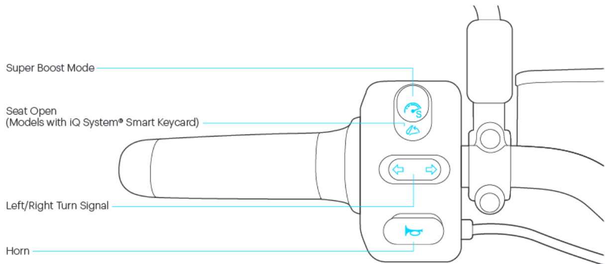
Left Handle (with 3 kW Motor)
